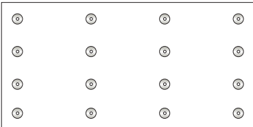
16 No. per board (2.4 x 1.2 m board – 5.55 fixings / m 2 )
