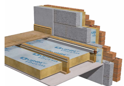
Suspended timber floor other than ground floor
