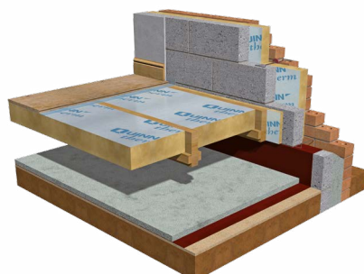
Suspended timber ground floor
