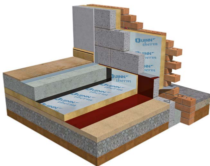
Solid ground floor: QF below groundbearing slab
