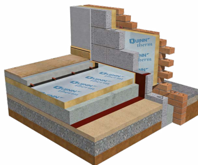
Solid ground floor: QF above groundbearing slab
