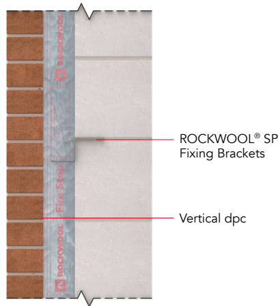
Figure 5 ROCKWOOL SP® Firestop Slab between masonry leaves
