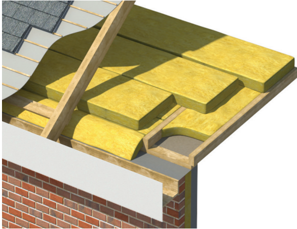
Lofts - Insulating between and over joists
