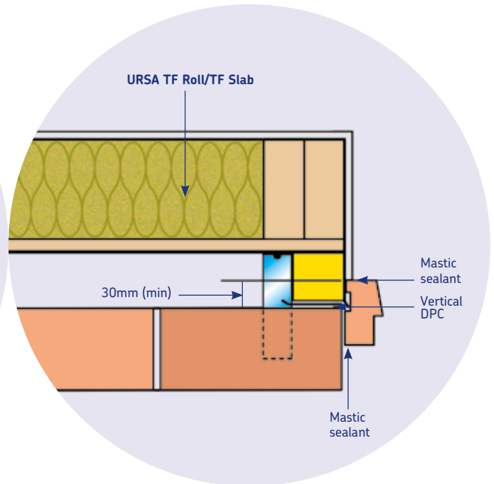
Figure 9 – Jamb Detail
