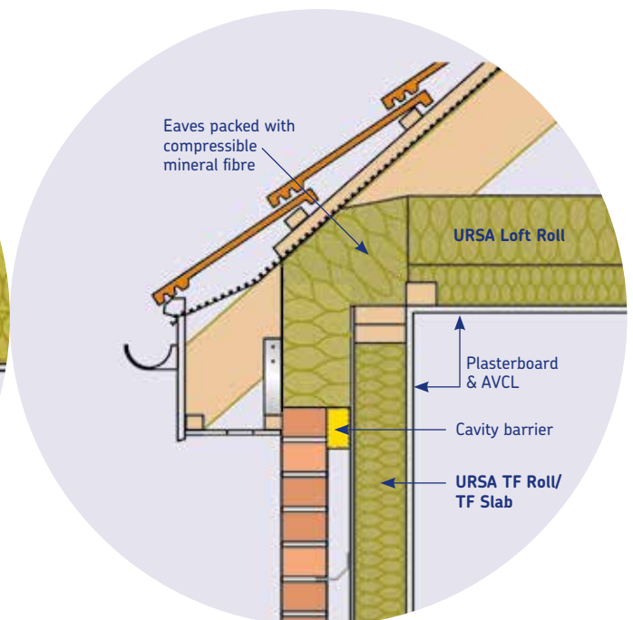
Figure 11 – Cold Pitched Roof – Eaves Detail
